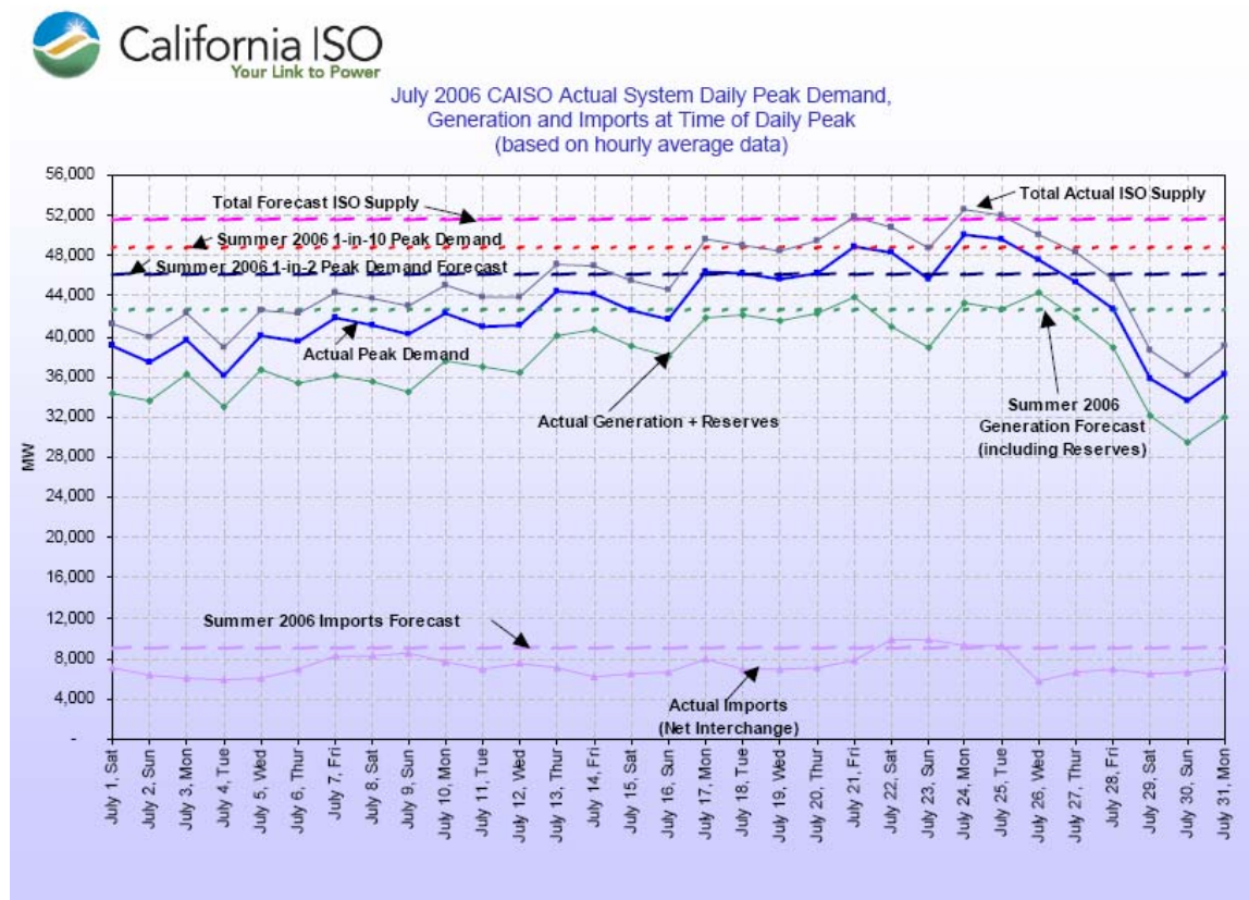
Figure 1 - System Daily Peak Demand July 2006
